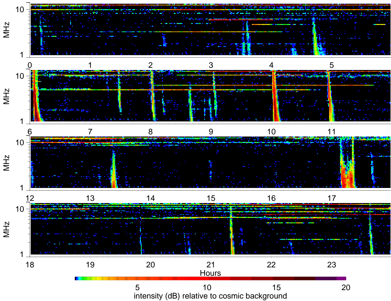
Wind Waves RAD2 receiver: 2000/7/3
