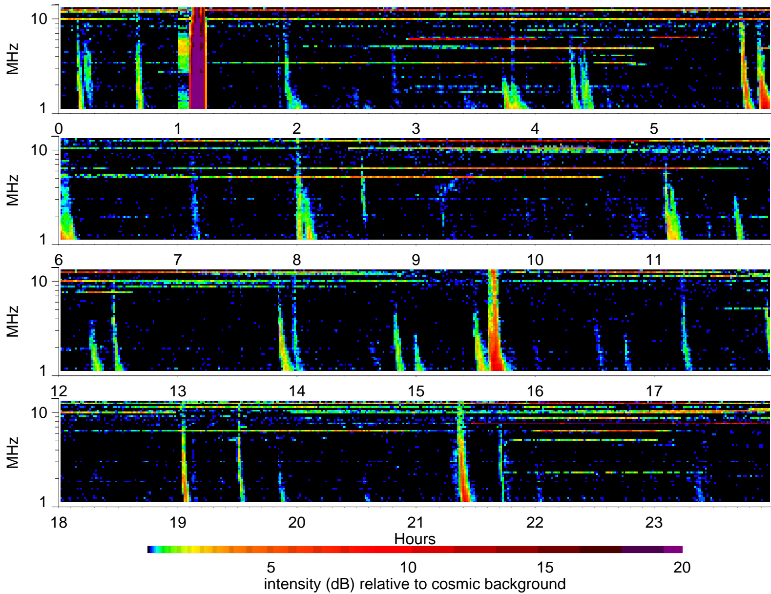
Wind Waves RAD2 receiver: 2000/7/2
