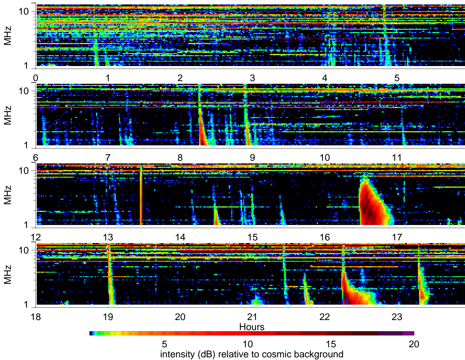
Wind Waves RAD2 receiver: 2000/6/27
