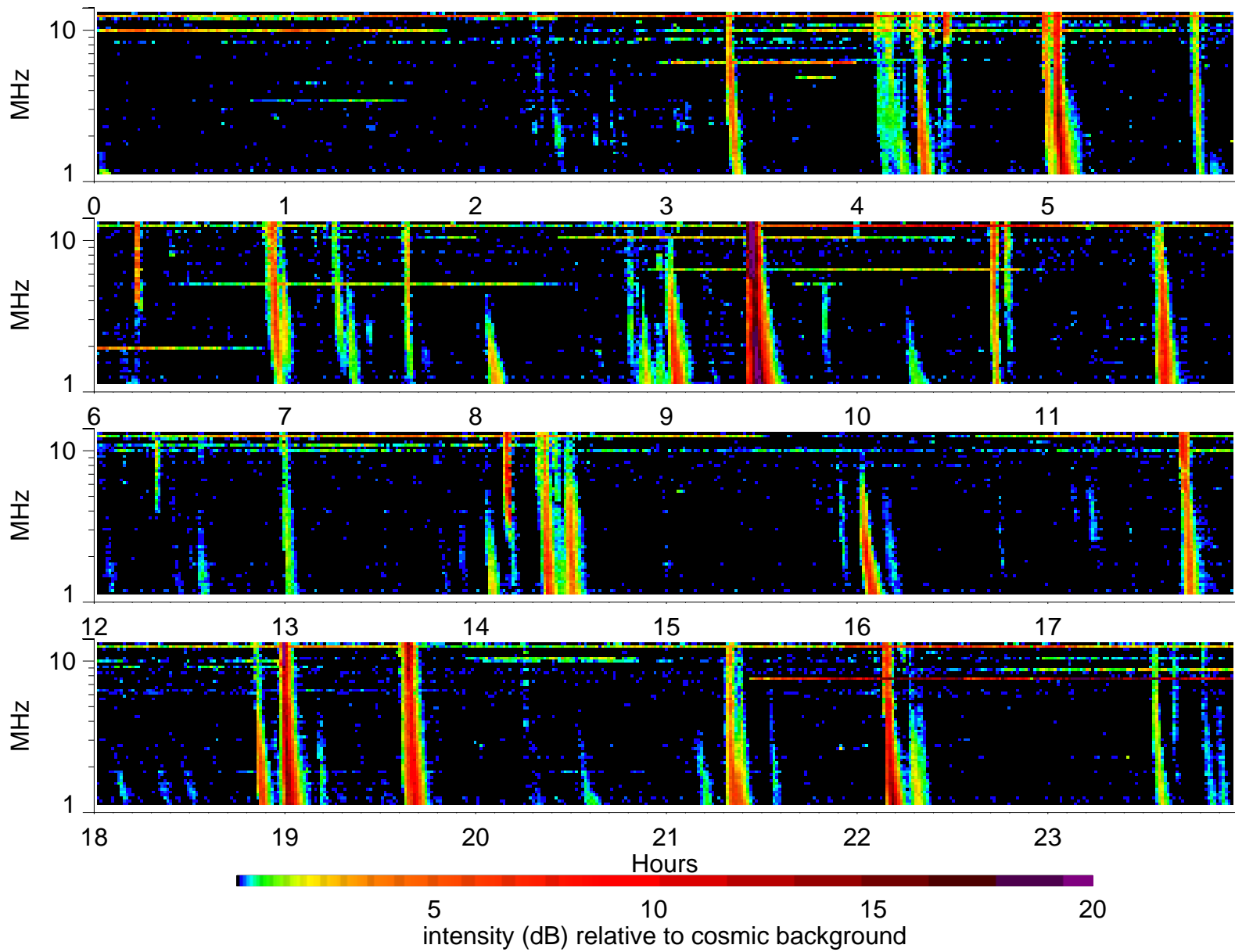
Wind Waves RAD2 receiver: 2000/6/21
