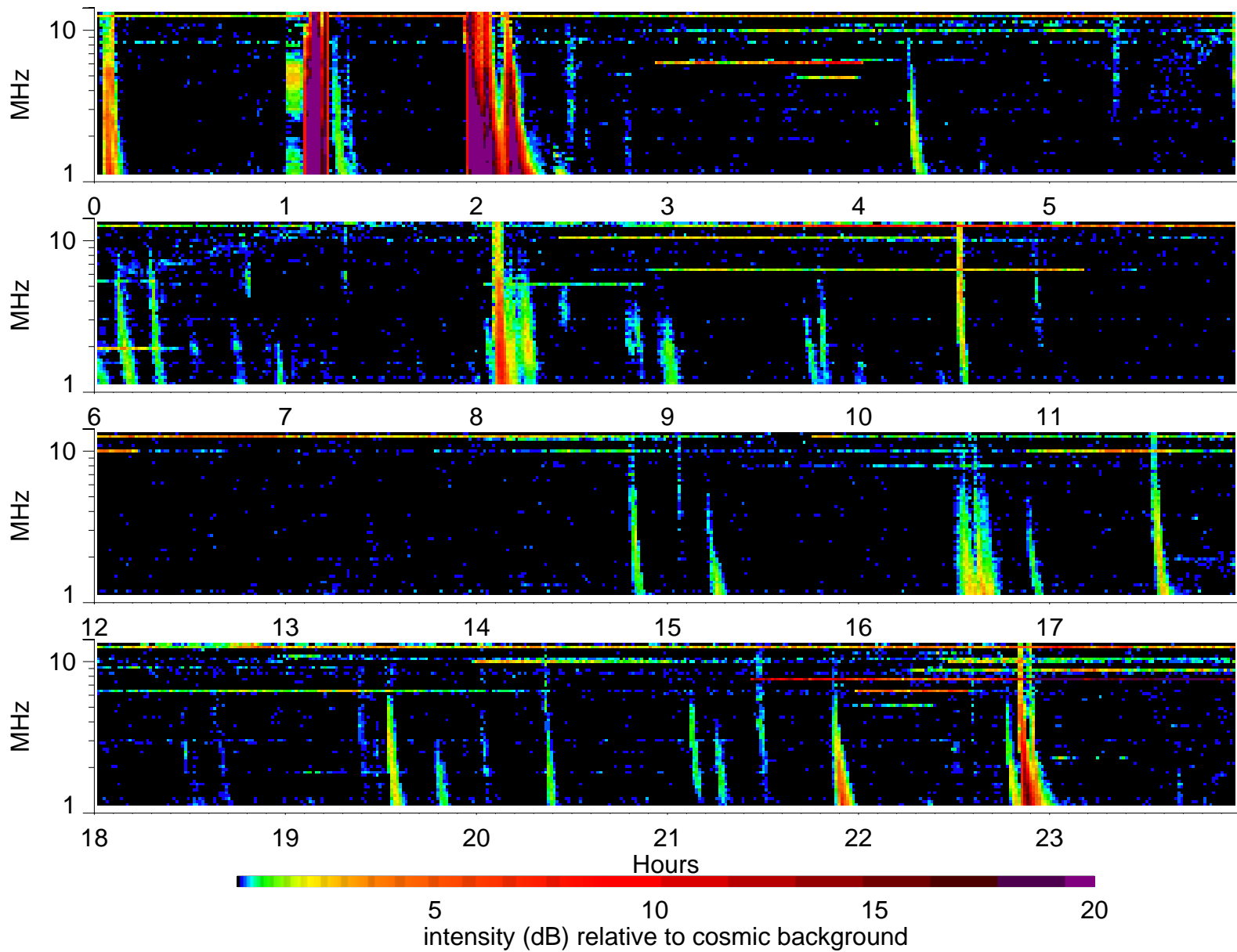
Wind Waves RAD2 receiver: 2000/6/18
