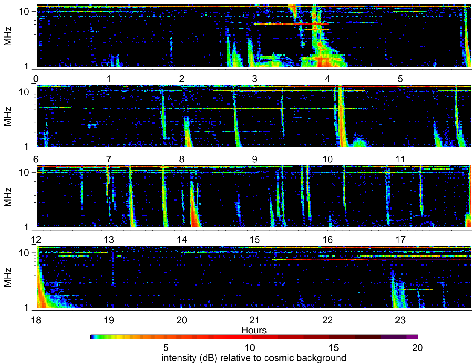
Wind Waves RAD2 receiver: 2000/6/17
