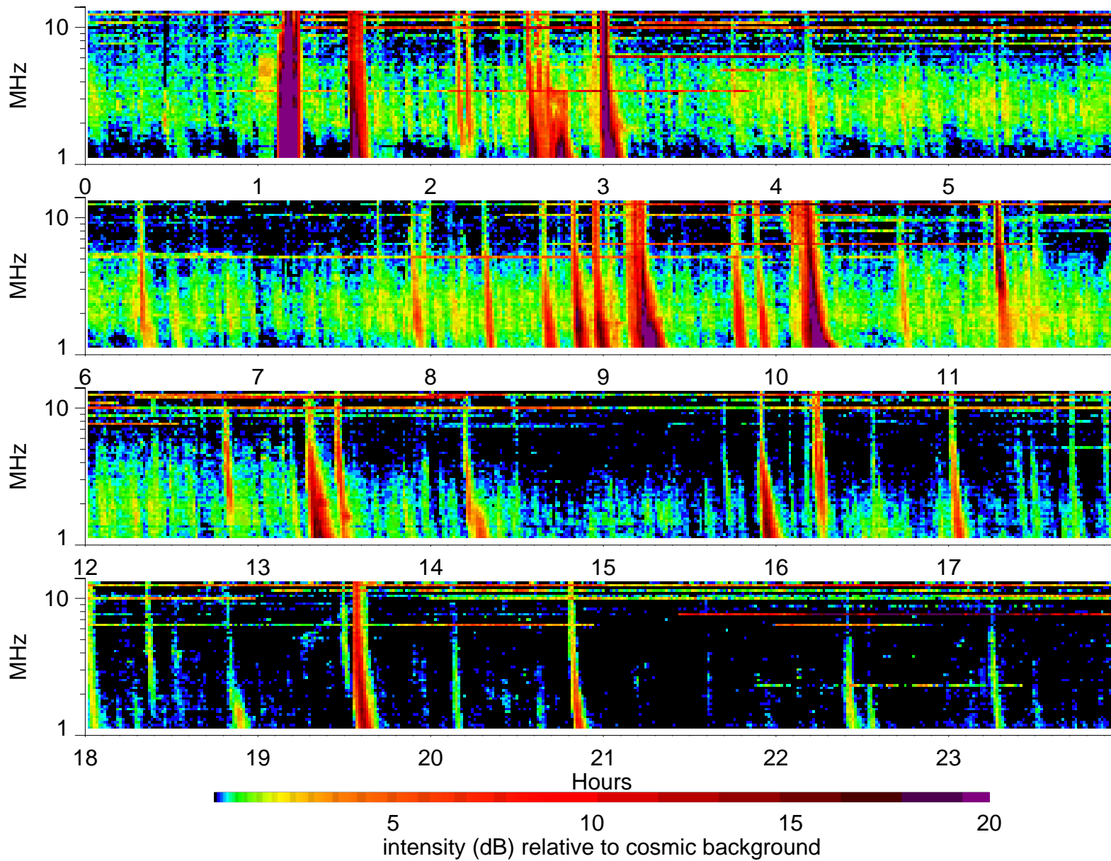
Wind Waves RAD2 receiver: 2000/6/12
