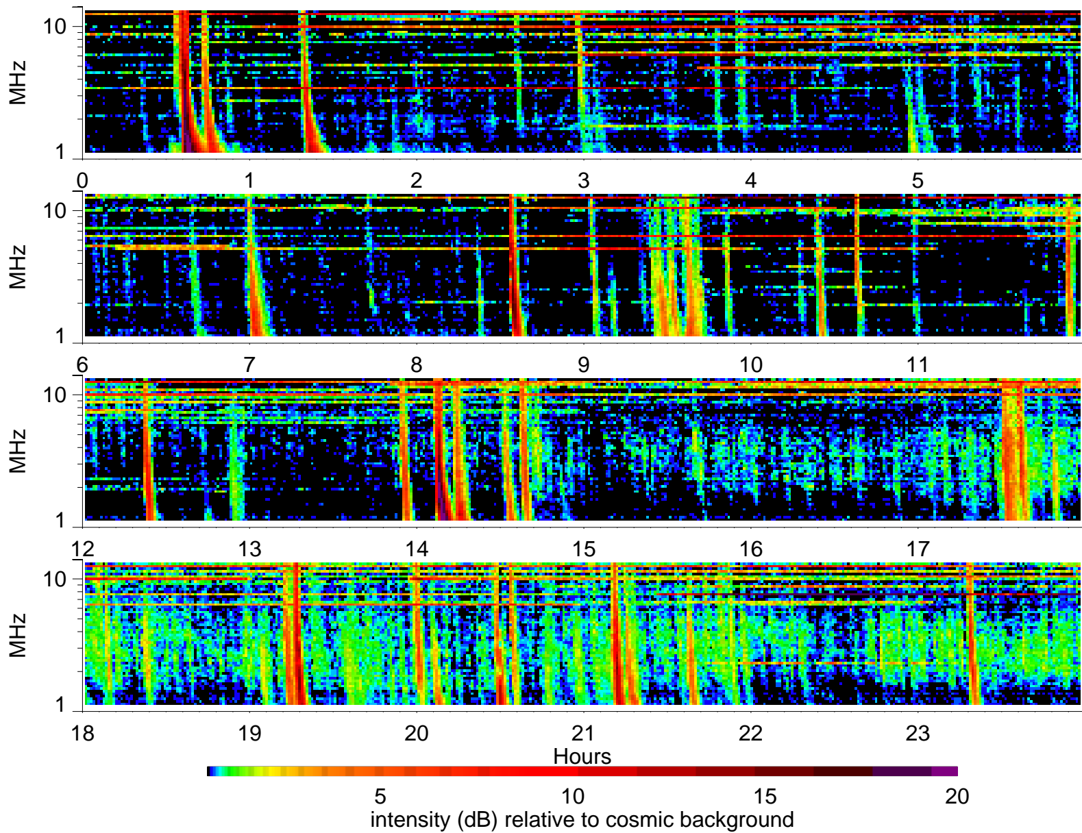
Wind Waves RAD2 receiver: 2000/6/11
