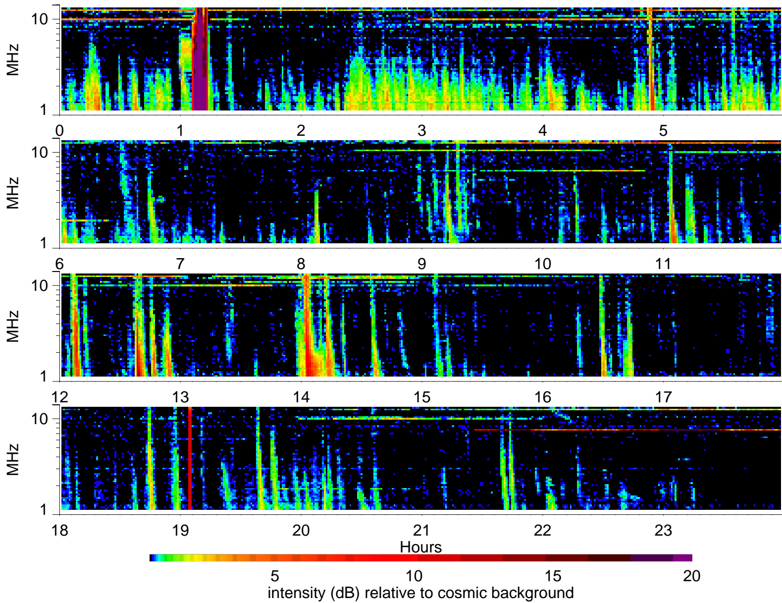
Wind Waves RAD2 receiver: 2000/6/2
