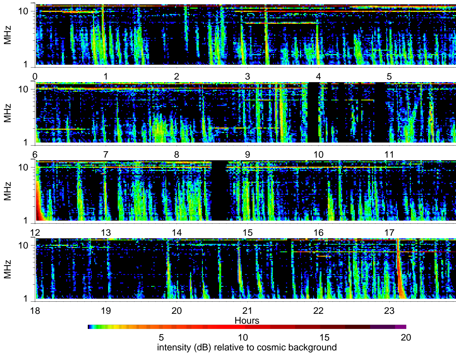
Wind Waves RAD2 receiver: 2000/5/30
