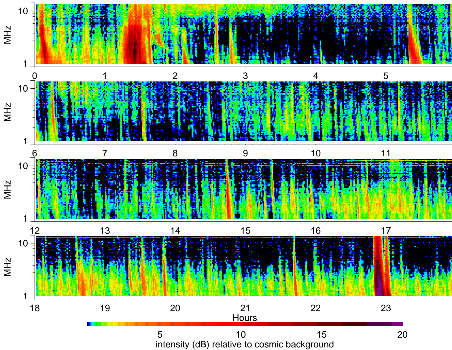
Wind Waves RAD2 receiver: 2000/5/22
