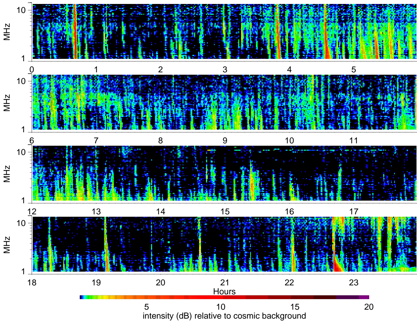
Wind Waves RAD2 receiver: 2000/5/20
