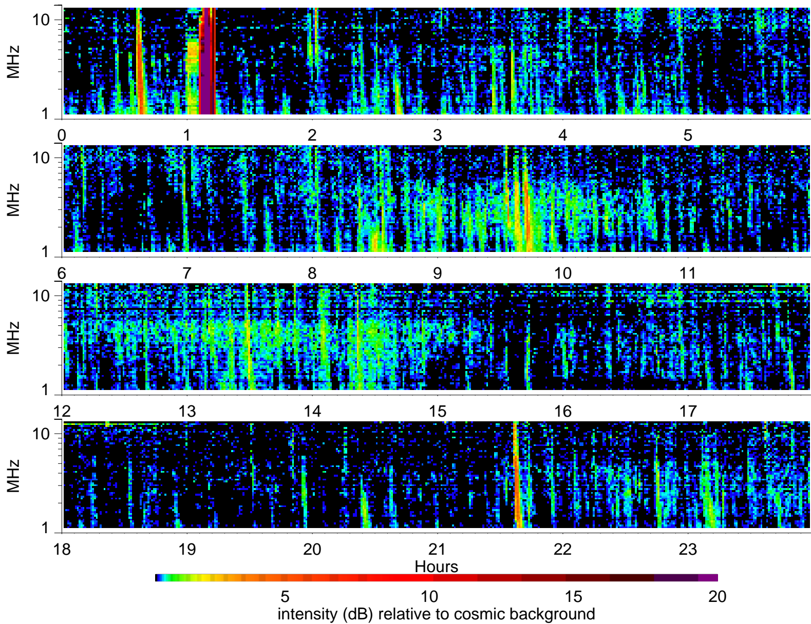
Wind Waves RAD2 receiver: 2000/5/19
