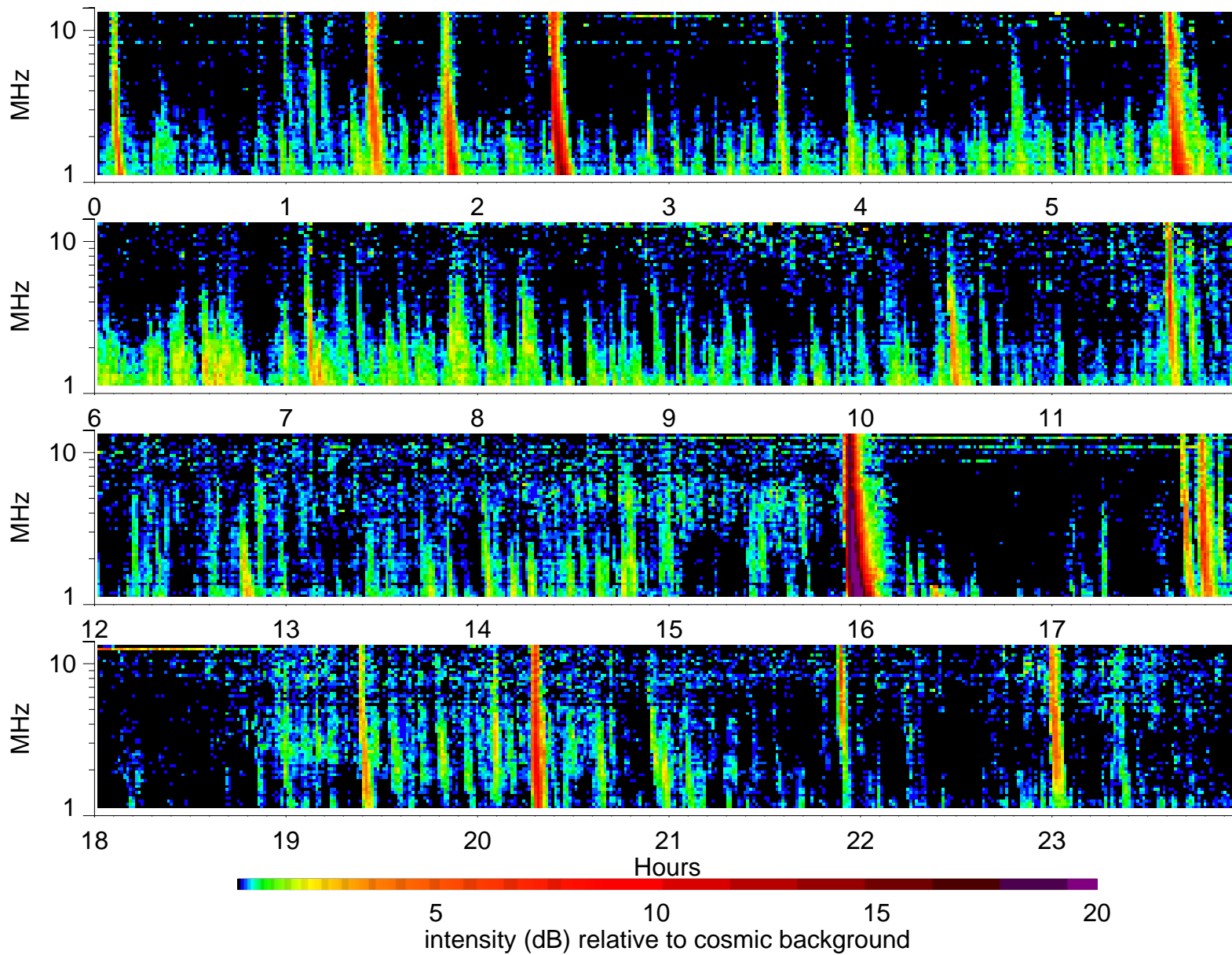
Wind Waves RAD2 receiver: 2000/5/18
