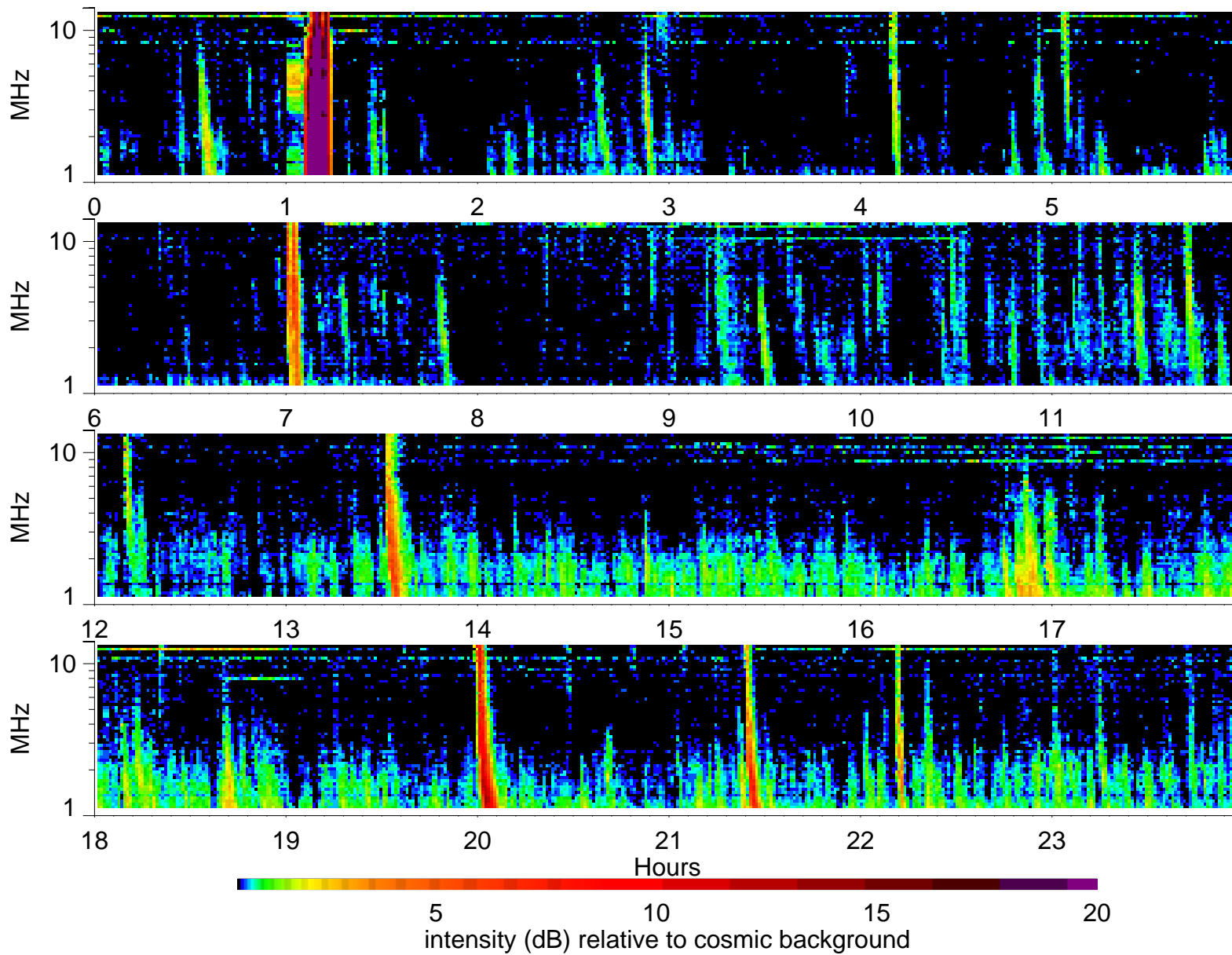
Wind Waves RAD2 receiver: 2000/5/17
