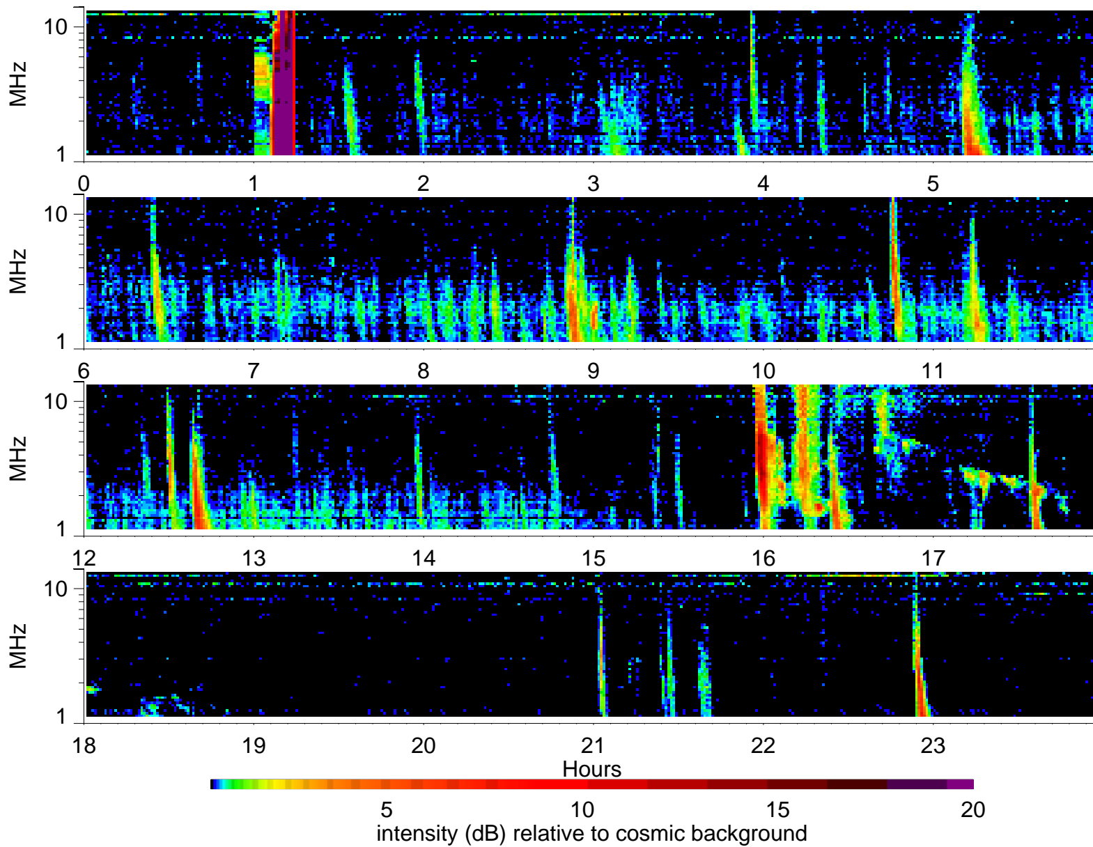
Wind Waves RAD2 receiver: 2000/5/15
