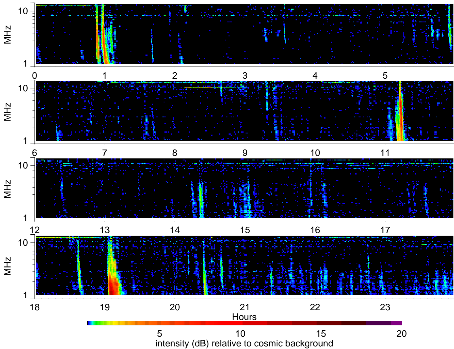
Wind Waves RAD2 receiver: 2000/5/14
