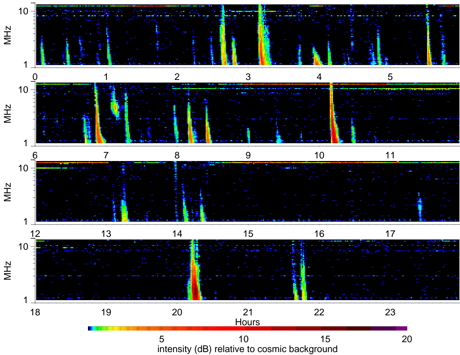
Wind Waves RAD2 receiver: 2000/5/6
