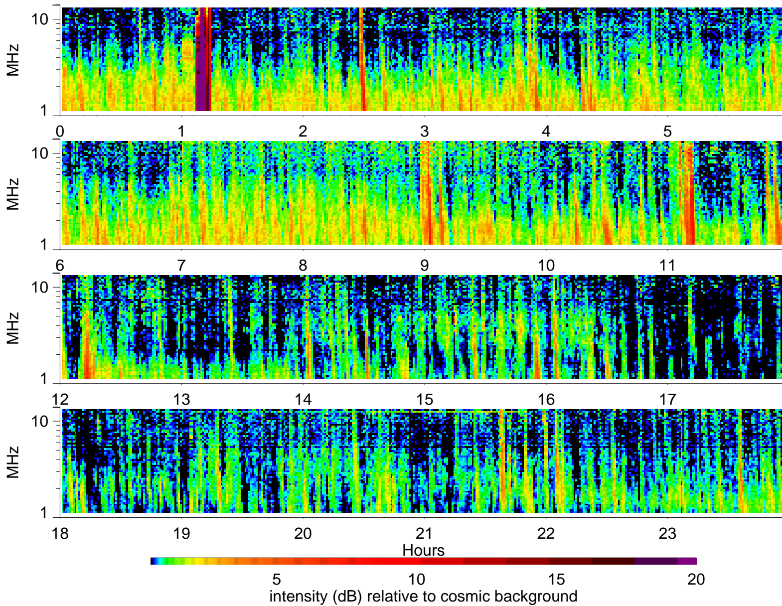
Wind Waves RAD2 receiver: 2000/4/29
