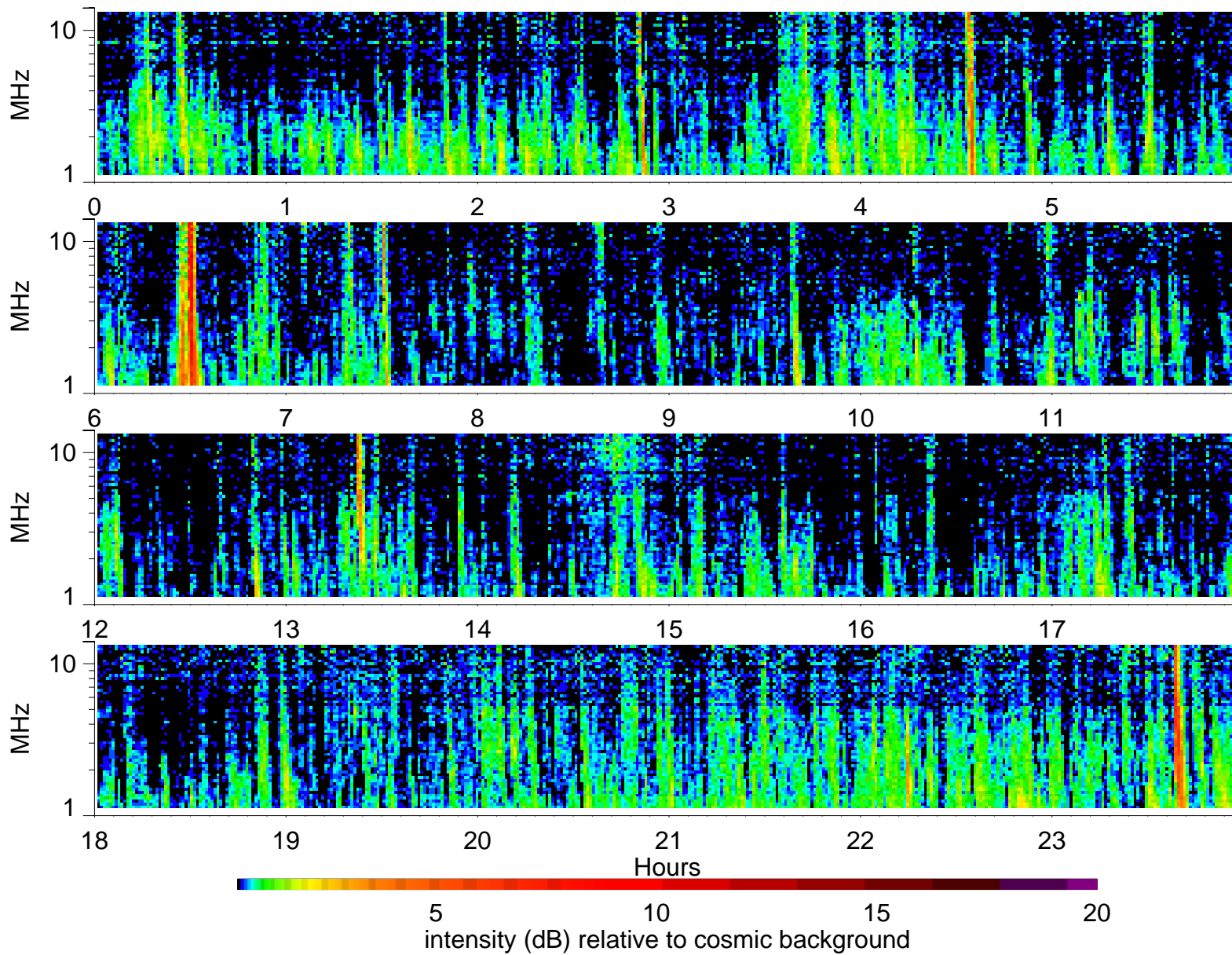
Wind Waves RAD2 receiver: 2000/4/26
