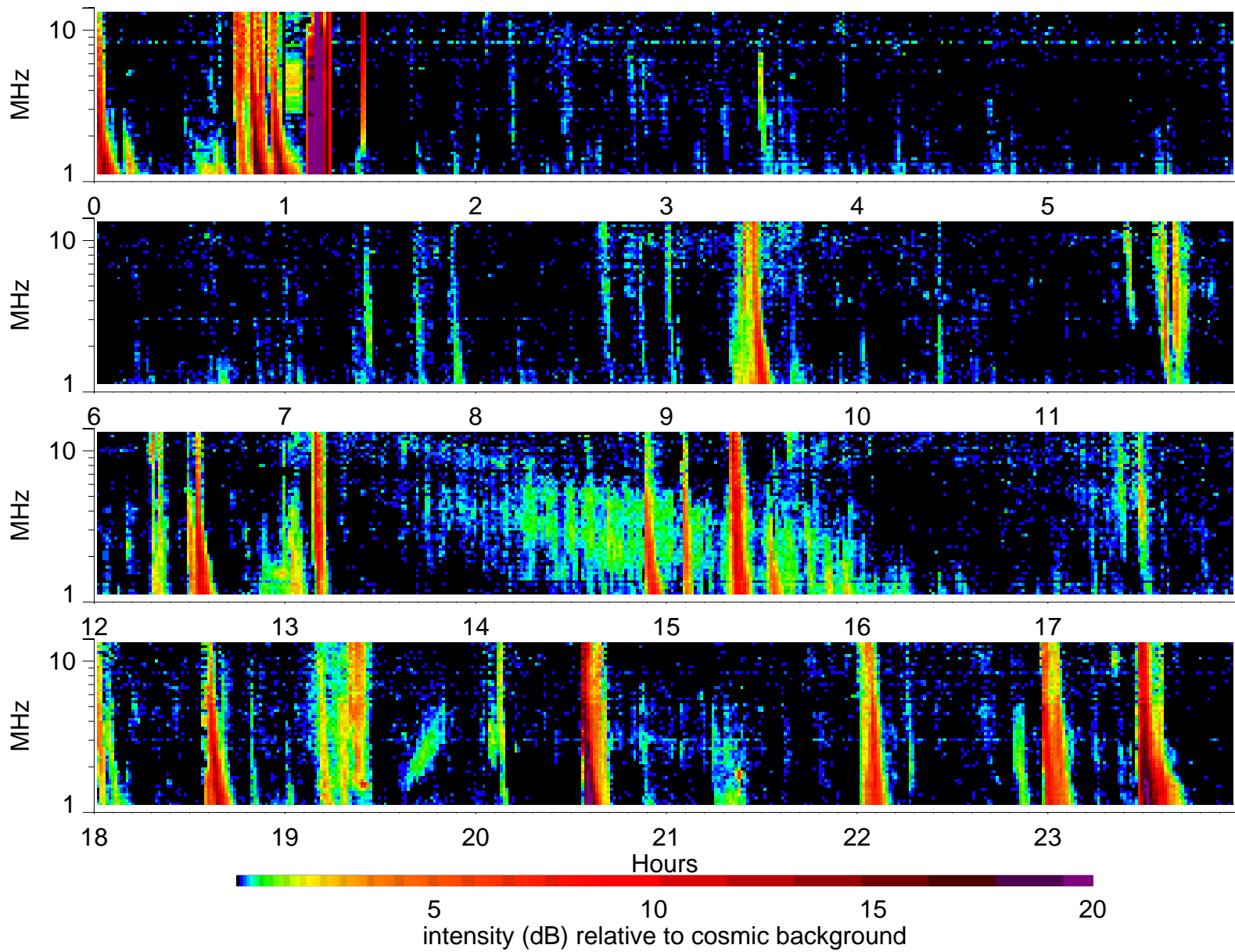
Wind Waves RAD2 receiver: 2000/4/21
