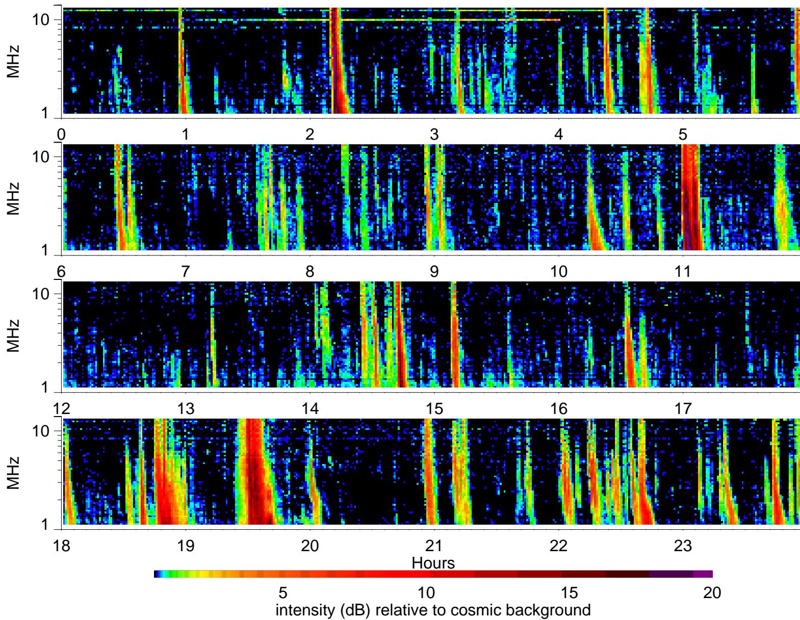
Wind Waves RAD2 receiver: 2000/4/20
