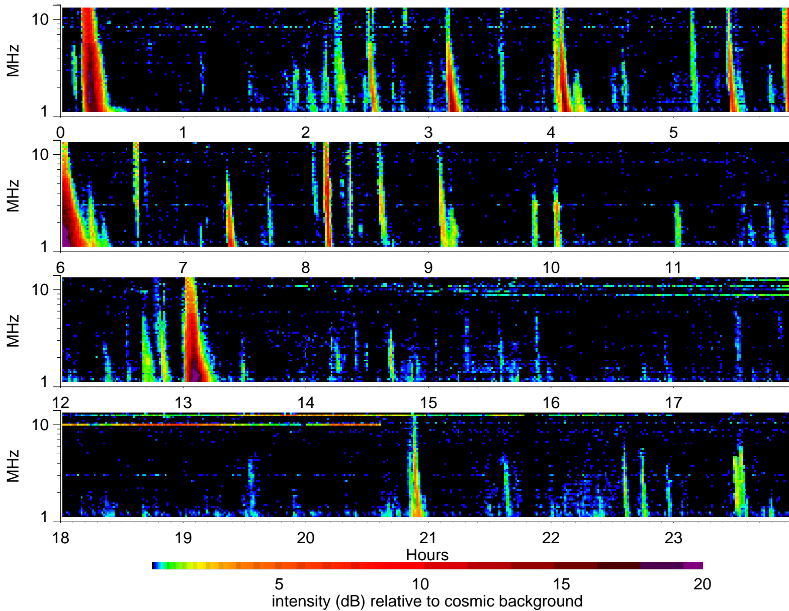
Wind Waves RAD2 receiver: 2000/4/16
