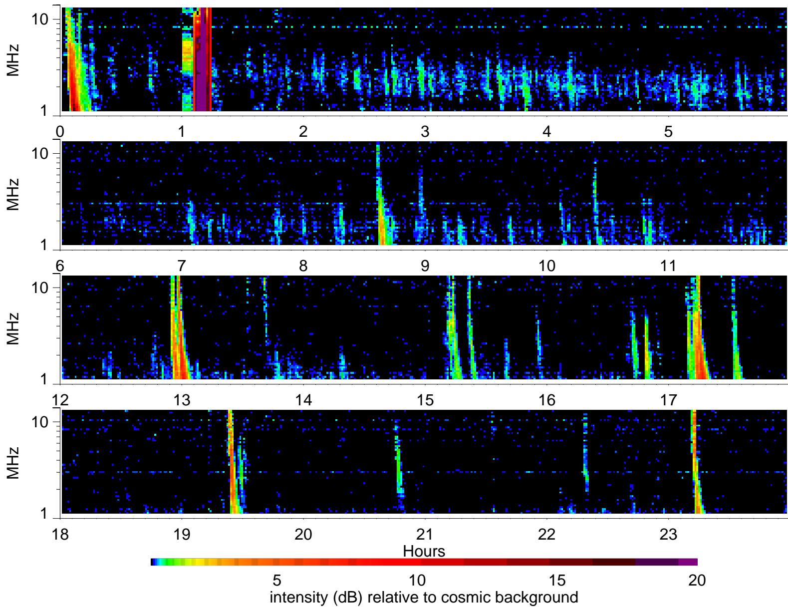
Wind Waves RAD2 receiver: 2000/4/13
