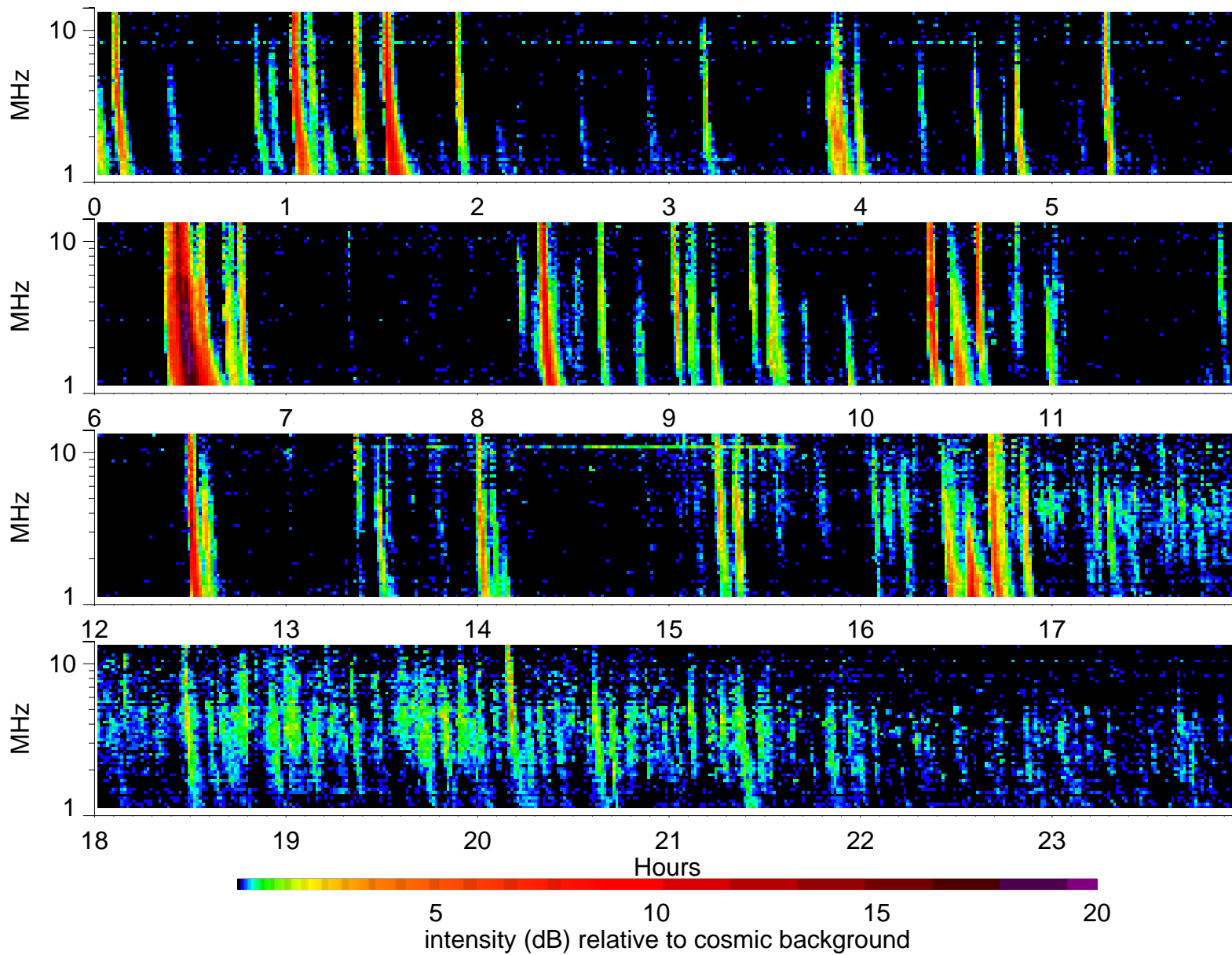
Wind Waves RAD2 receiver: 2000/4/12
