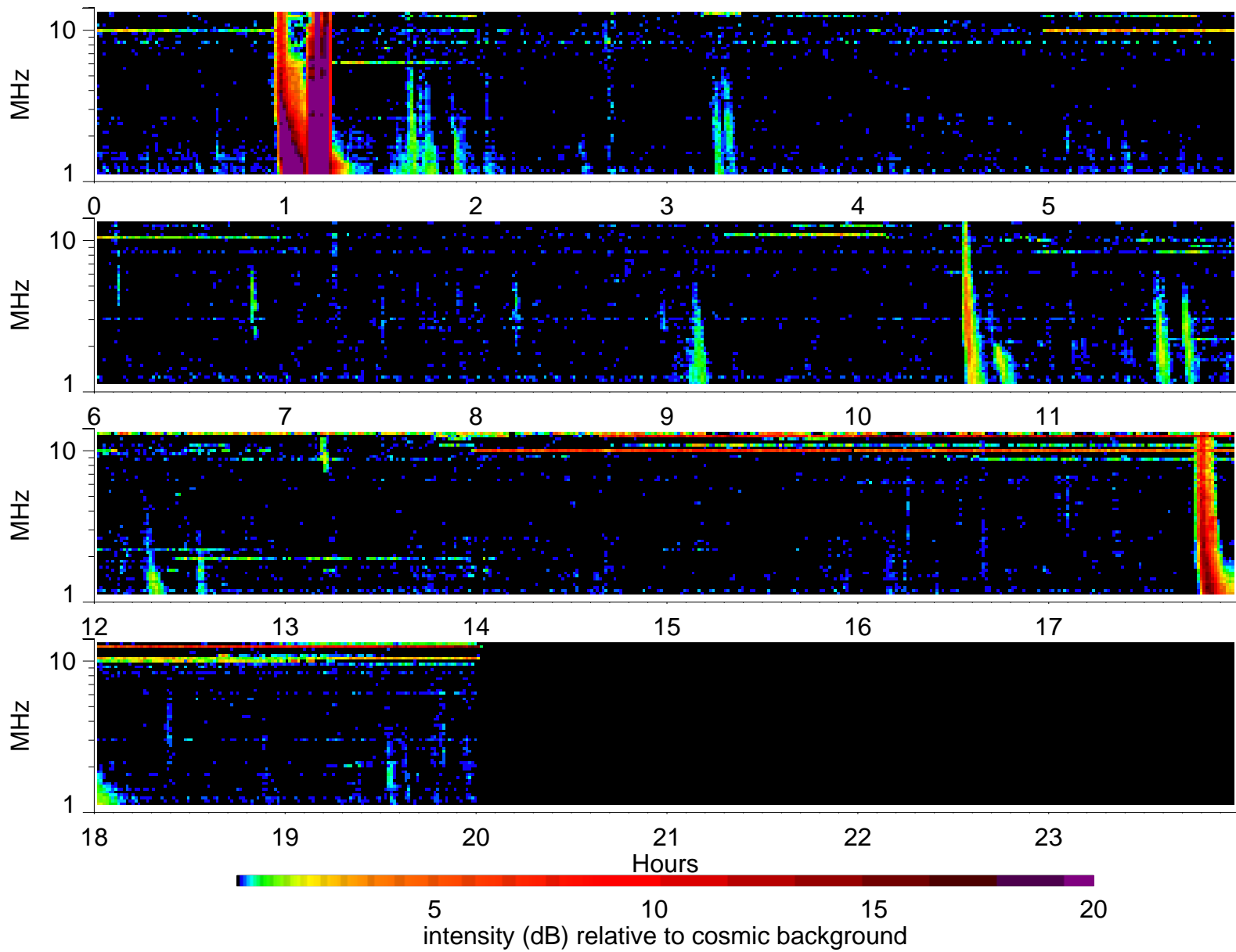
Wind Waves RAD2 receiver: 2000/4/7
