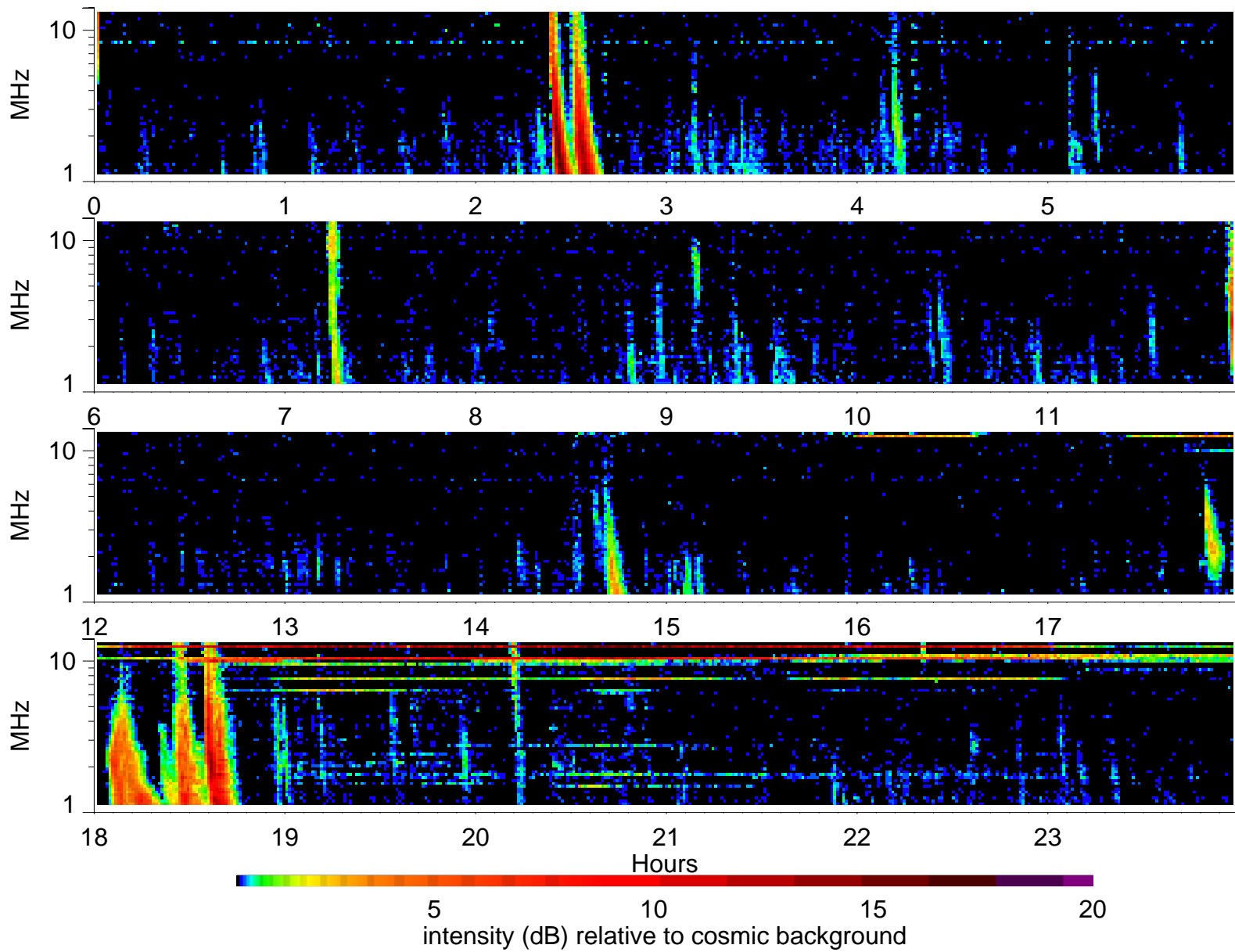
Wind Waves RAD2 receiver: 2000/4/6
