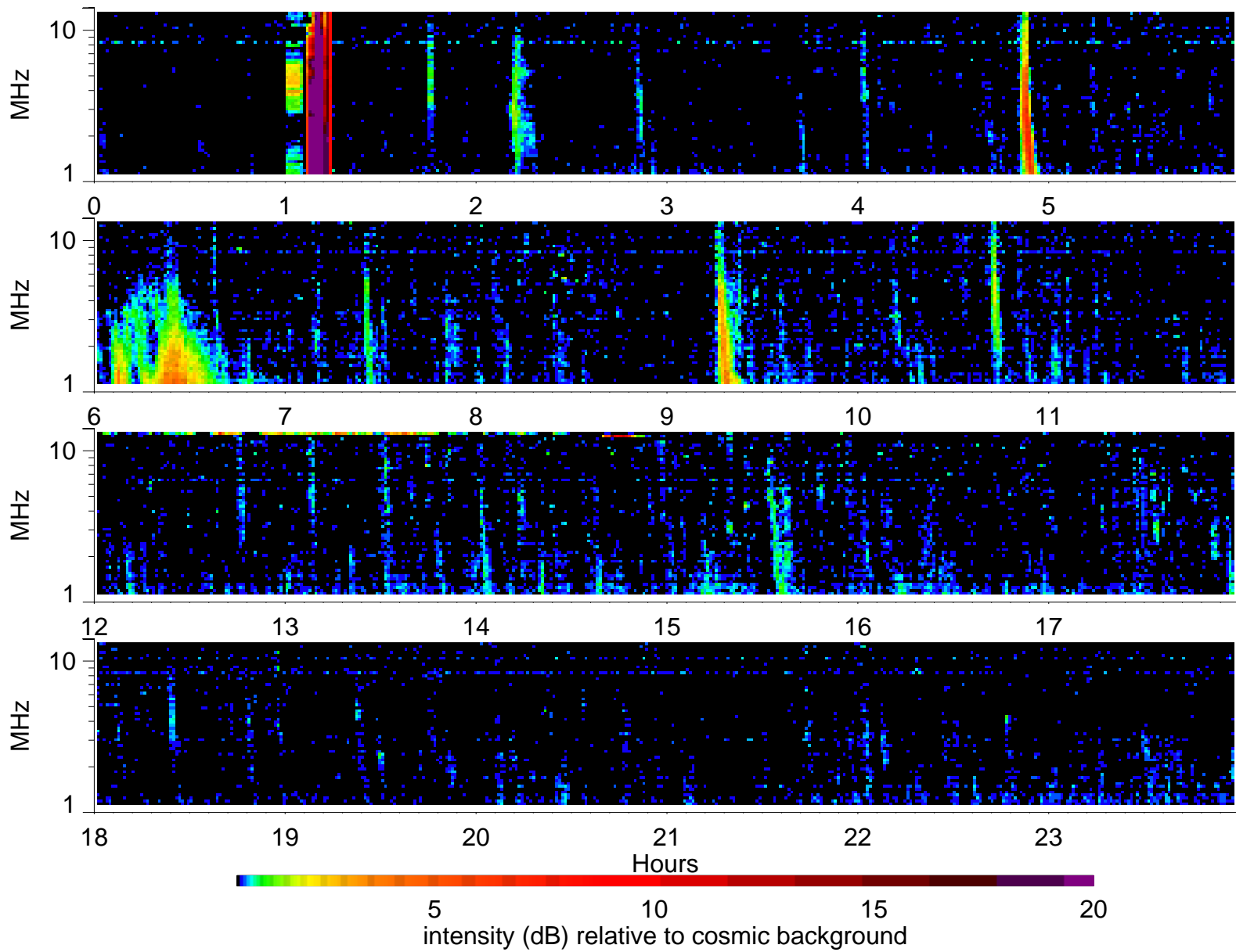
Wind Waves RAD2 receiver: 2000/4/5
