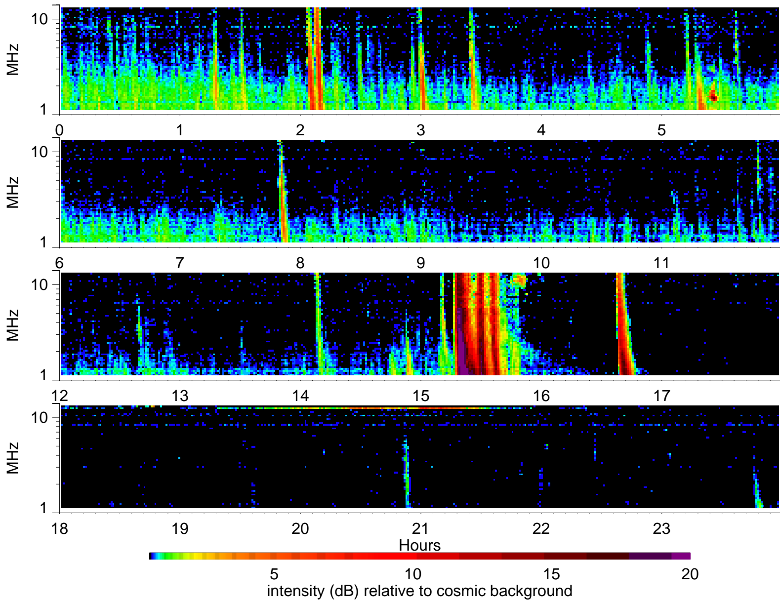
Wind Waves RAD2 receiver: 2000/4/4
