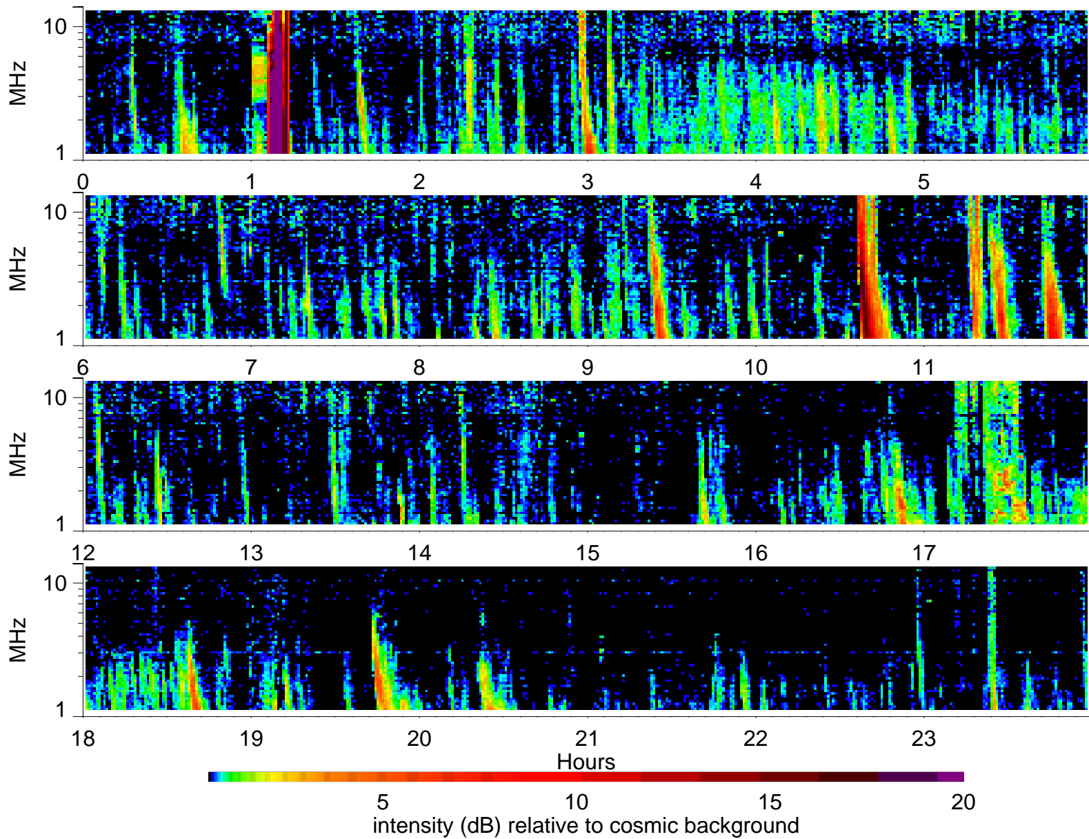
Wind Waves RAD2 receiver: 2000/3/26
