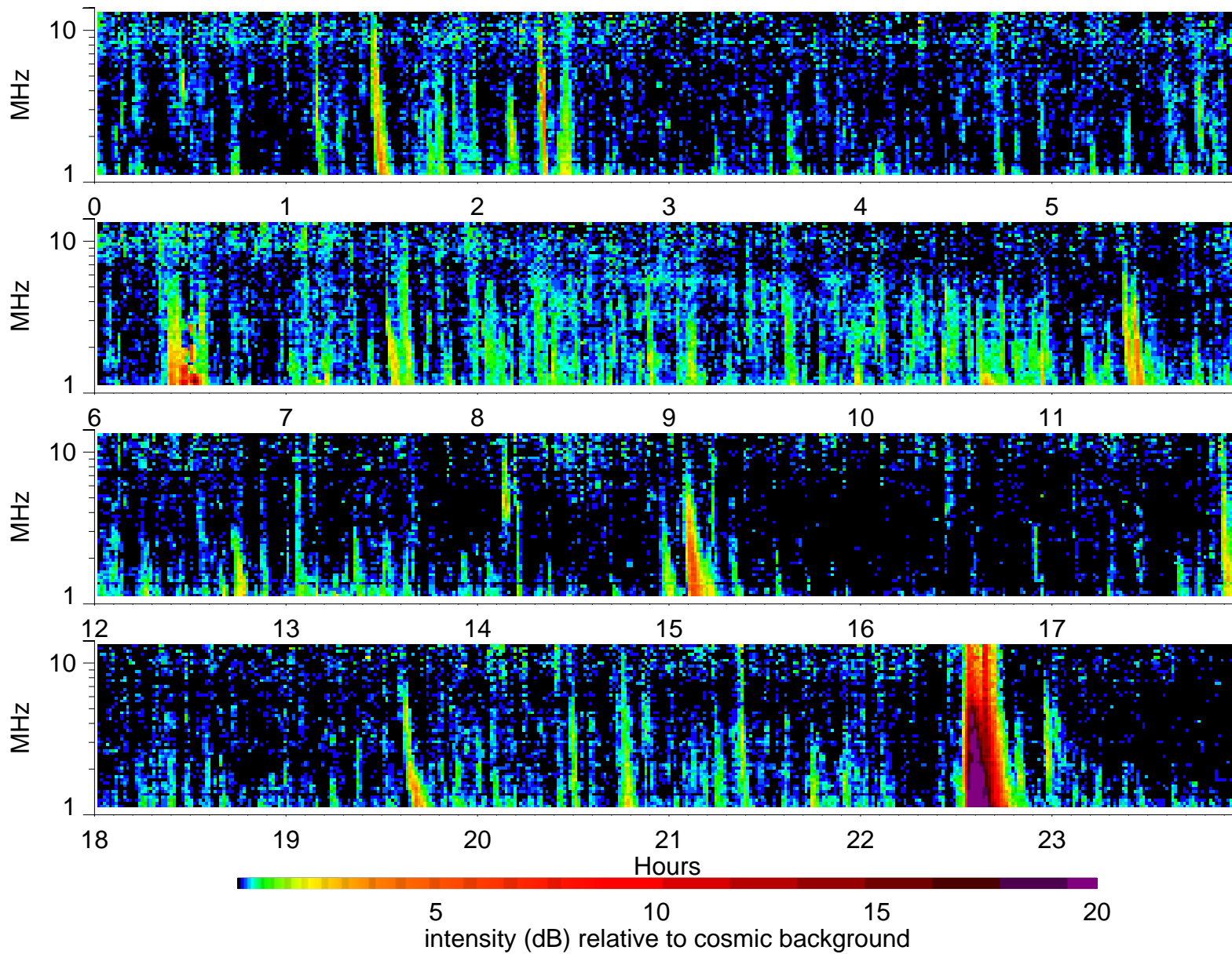
Wind Waves RAD2 receiver: 2000/3/25
