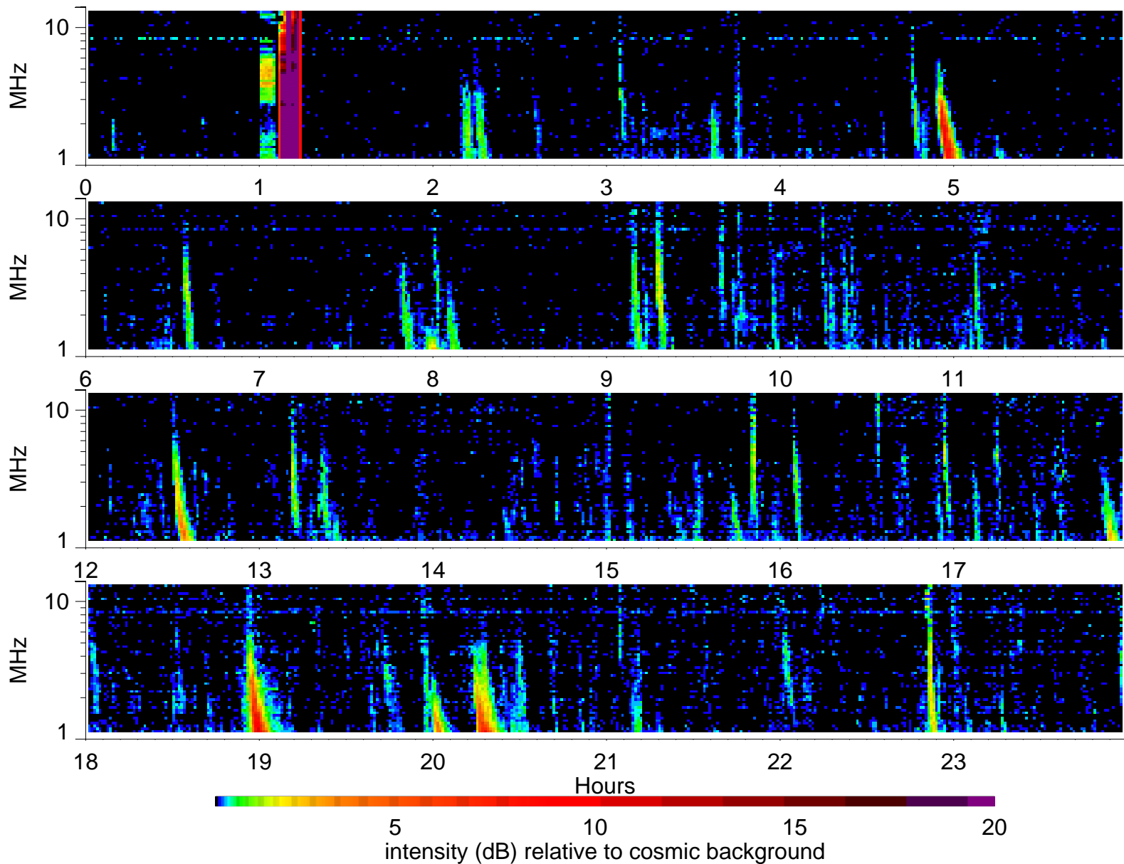
Wind Waves RAD2 receiver: 2000/3/22
