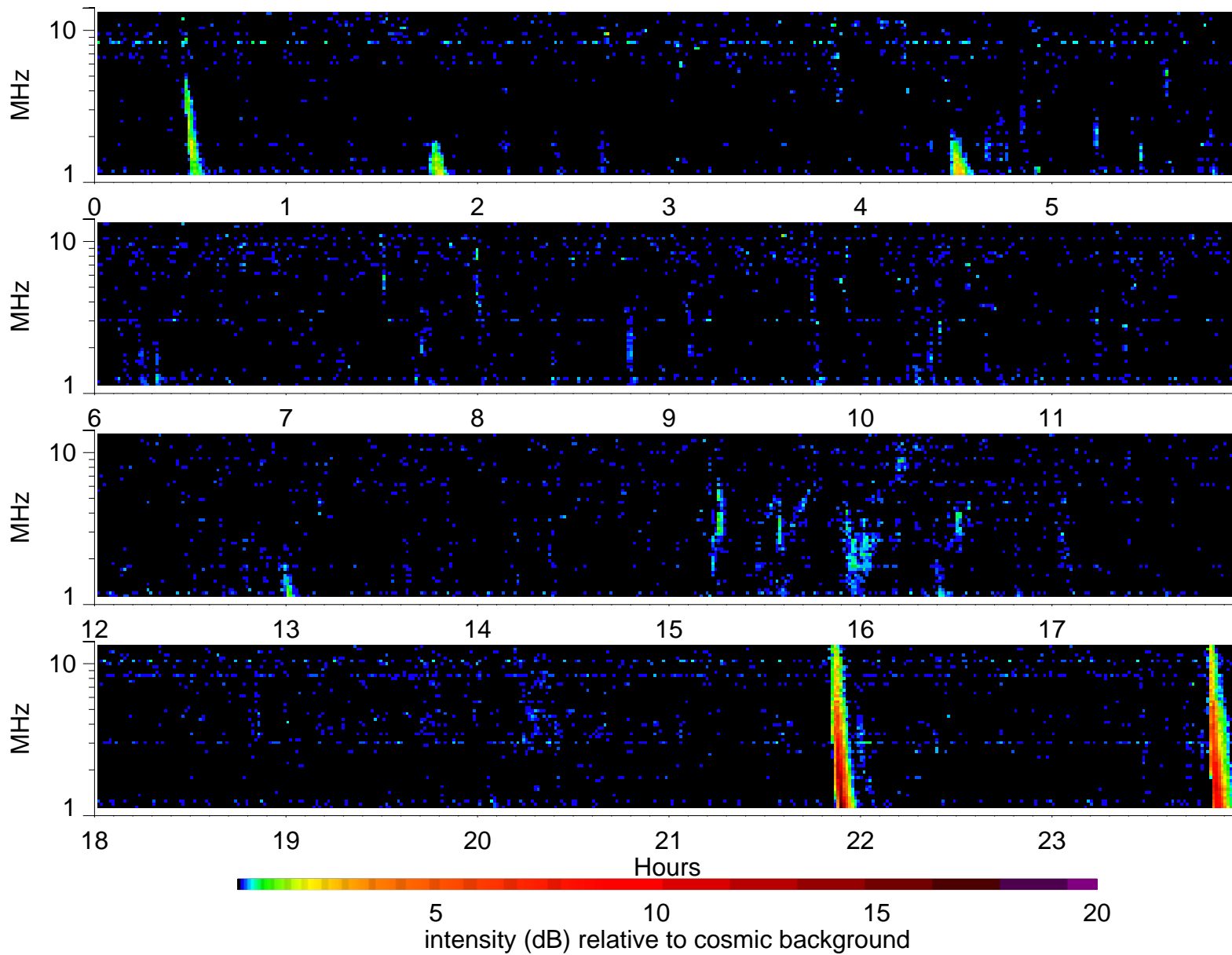
Wind Waves RAD2 receiver: 2000/3/11
