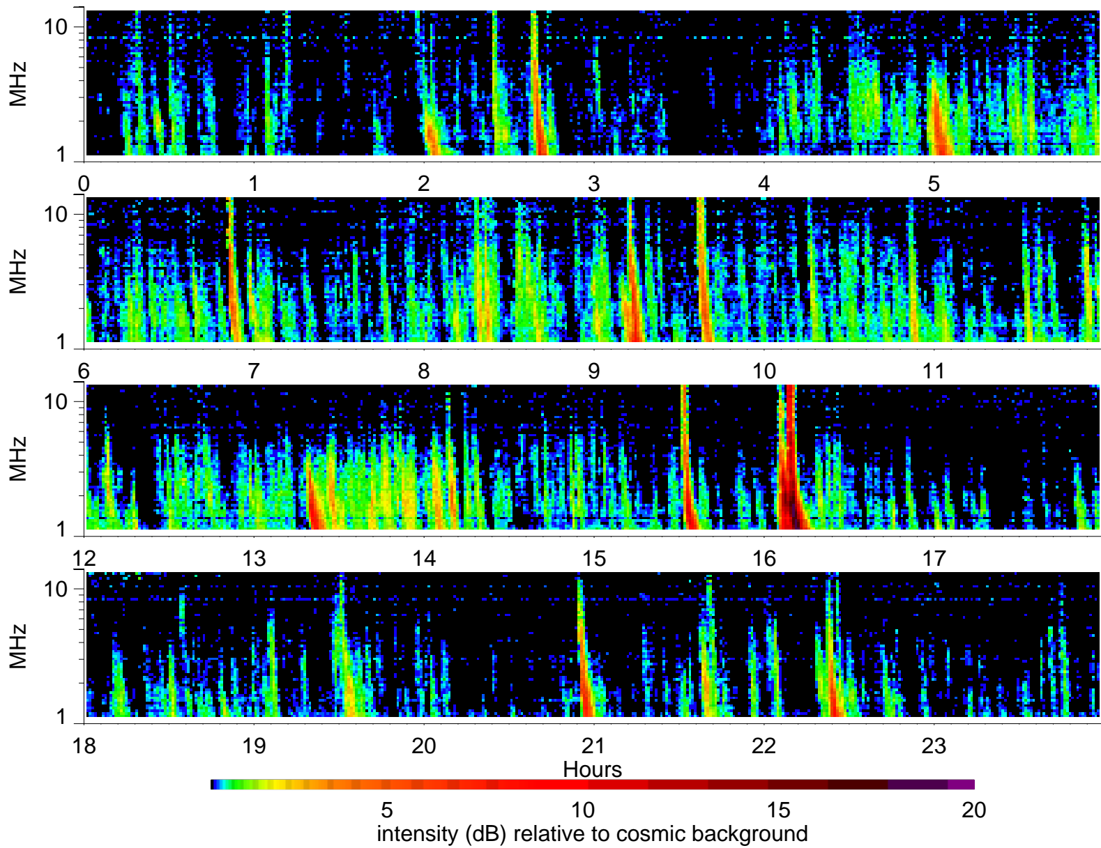
Wind Waves RAD2 receiver: 2000/3/5
