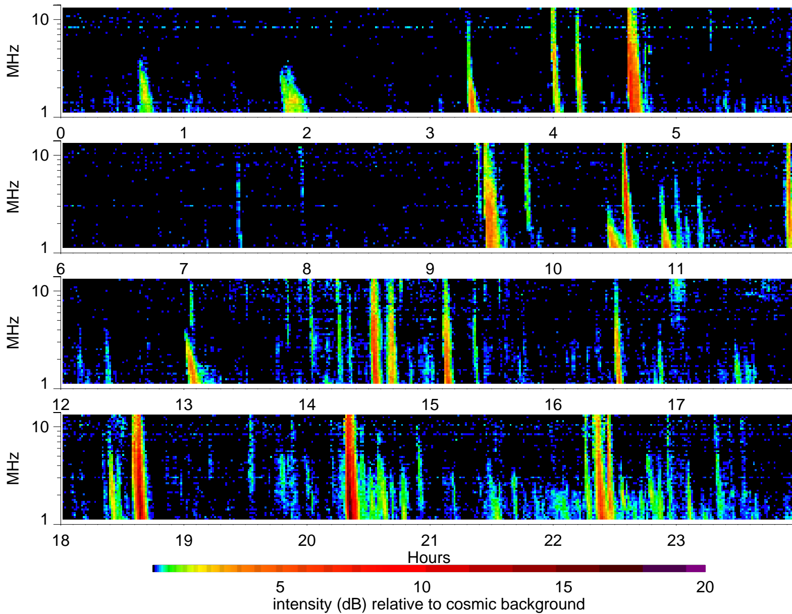
Wind Waves RAD2 receiver: 2000/2/28
