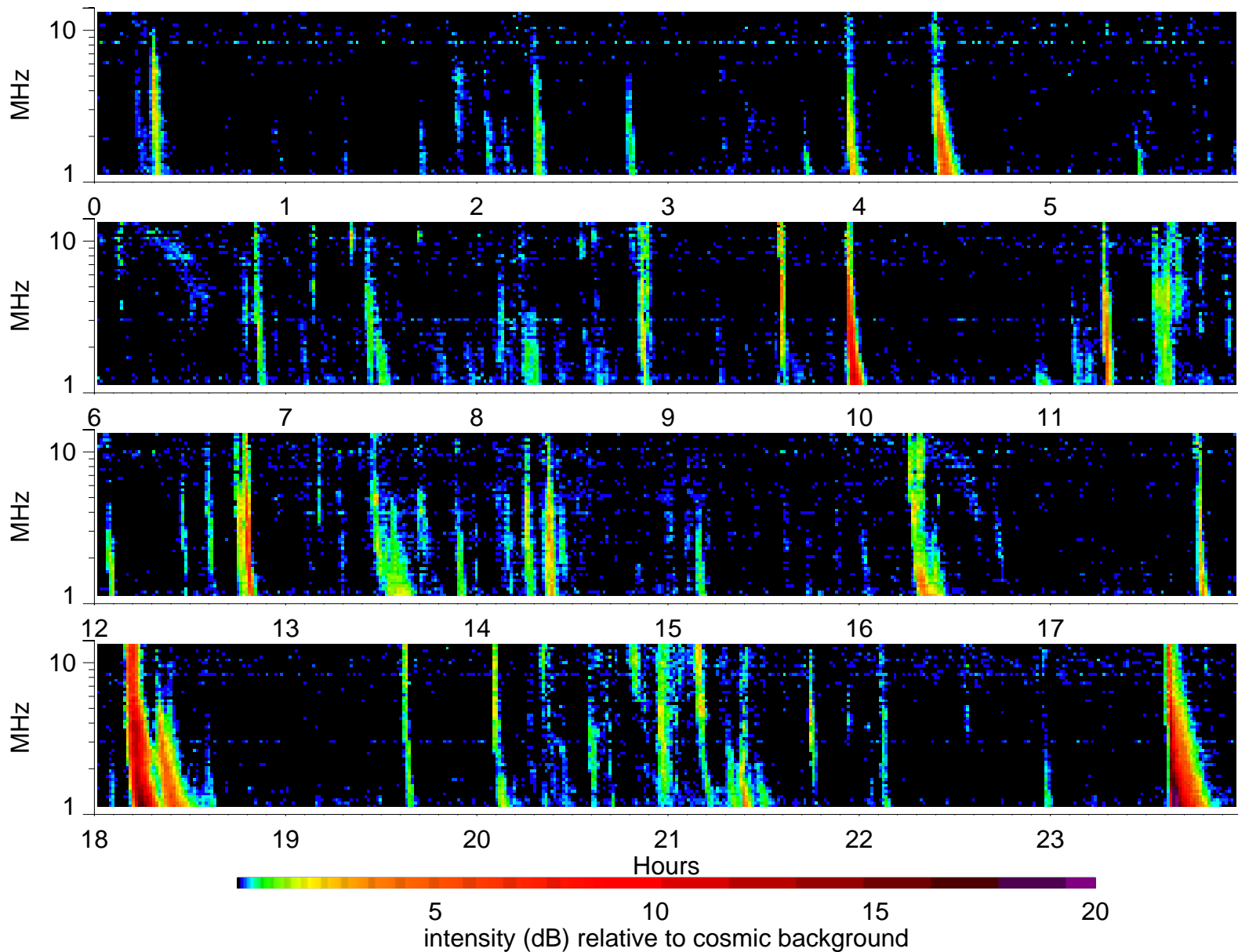
Wind Waves RAD2 receiver: 2000/2/26
