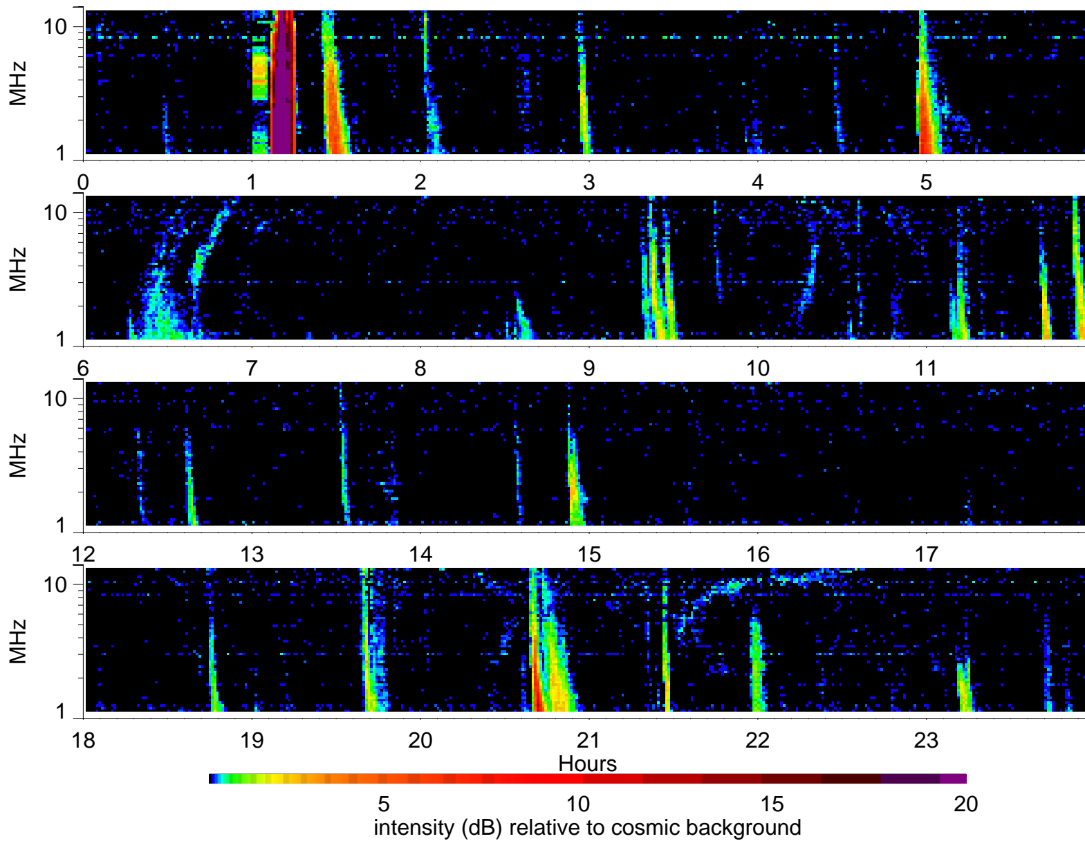
Wind Waves RAD2 receiver: 2000/2/25
