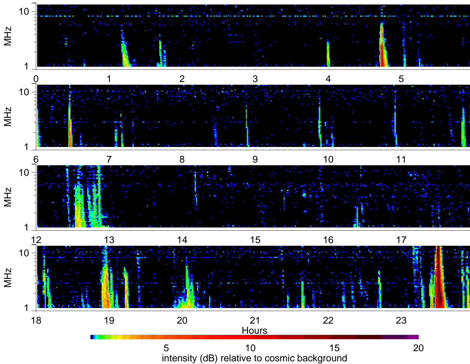
Wind Waves RAD2 receiver: 2000/2/22
