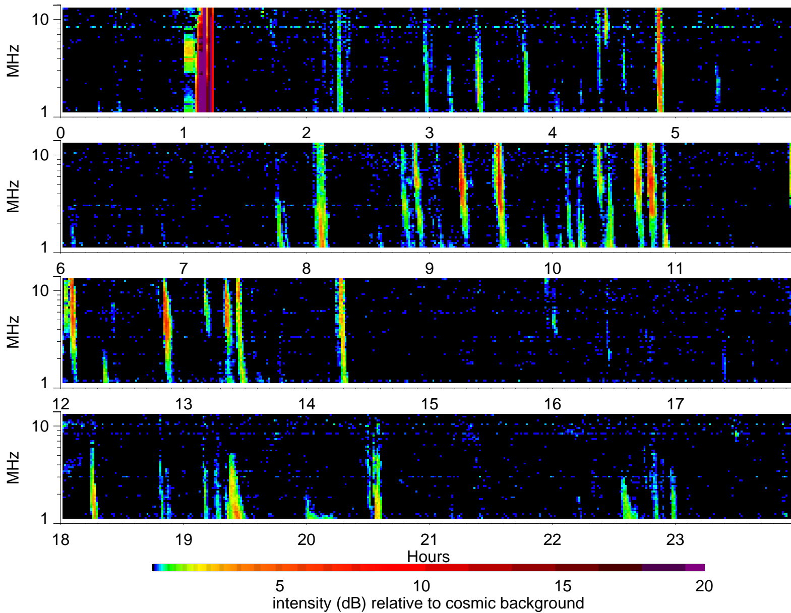
Wind Waves RAD2 receiver: 2000/2/21
