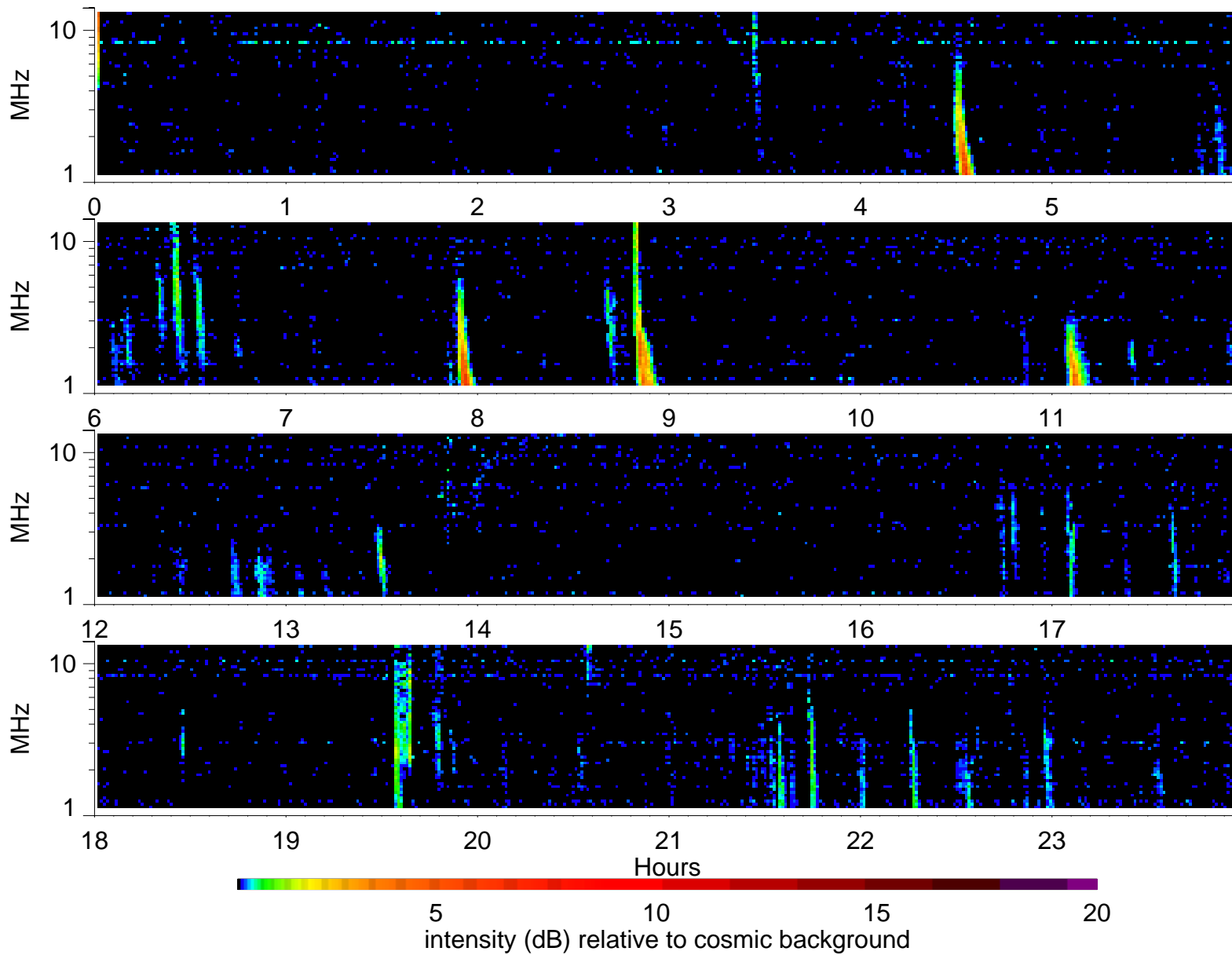
Wind Waves RAD2 receiver: 2000/2/20
