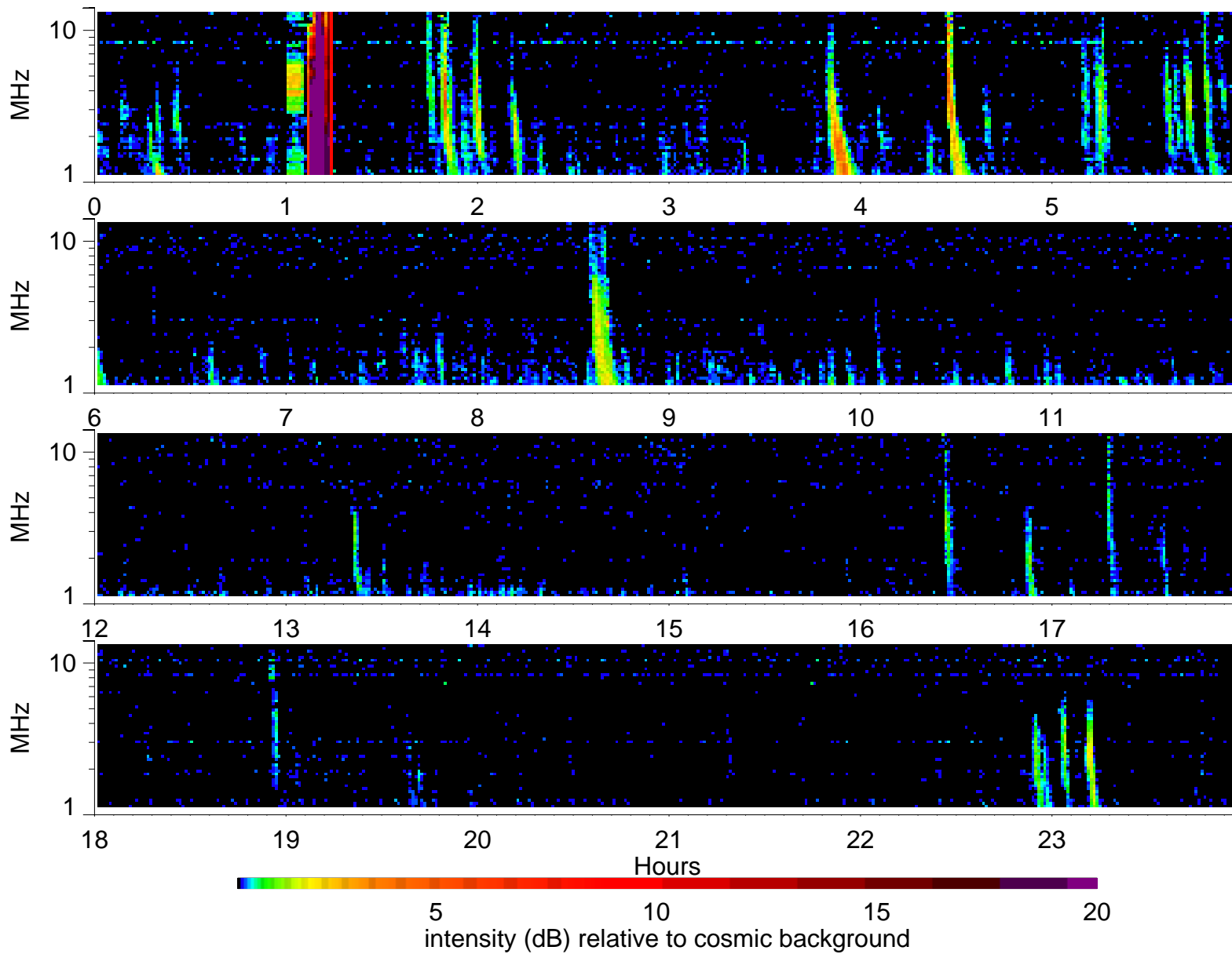
Wind Waves RAD2 receiver: 2000/2/19
