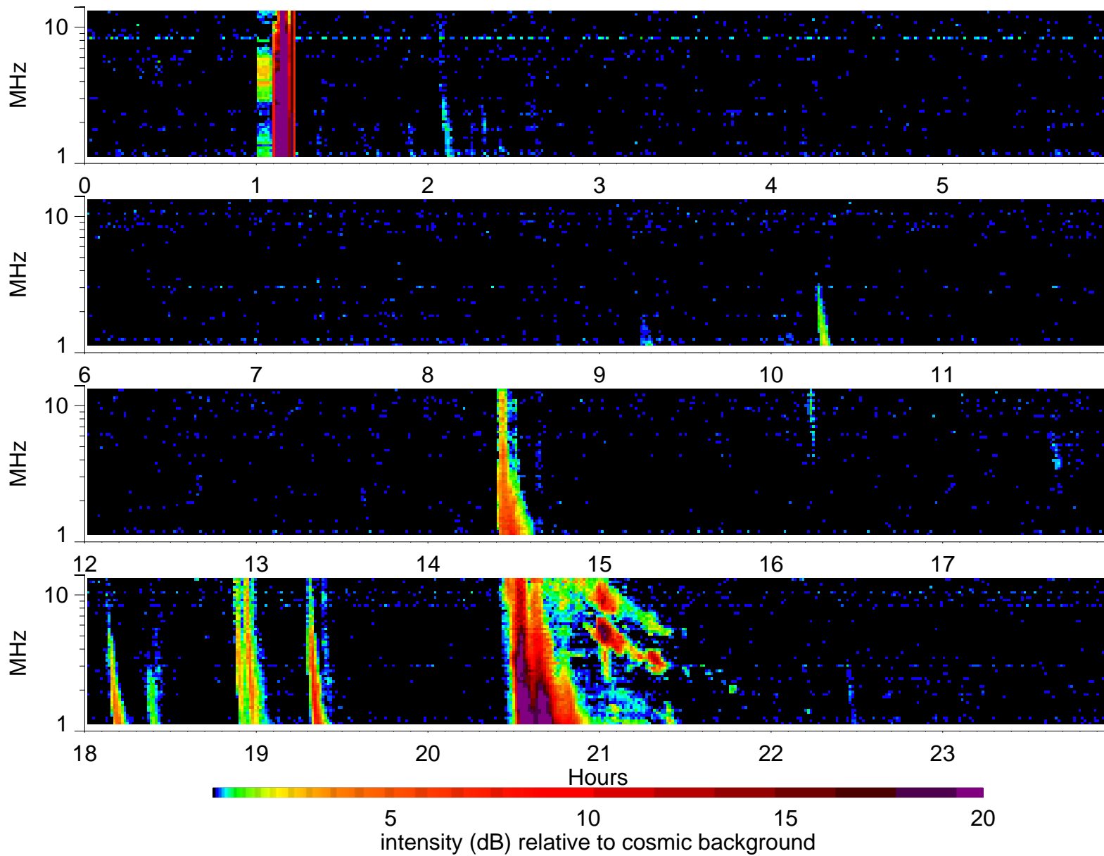
Wind Waves RAD2 receiver: 2000/2/17
