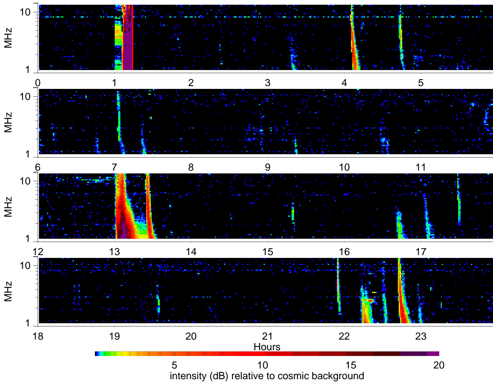
Wind Waves RAD2 receiver: 2000/2/13
