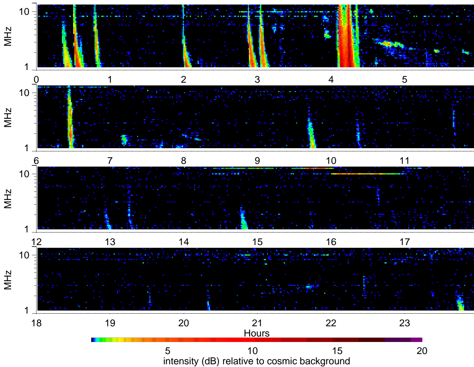
Wind Waves RAD2 receiver: 2000/2/12
