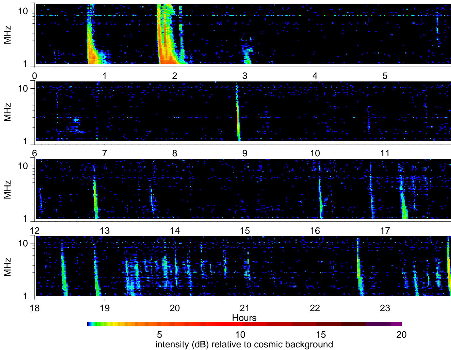
Wind Waves RAD2 receiver: 2000/2/10
