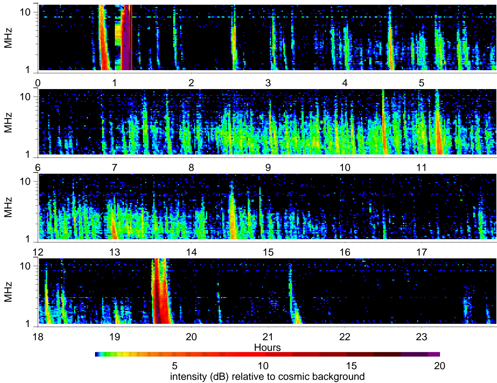
Wind Waves RAD2 receiver: 2000/2/9
