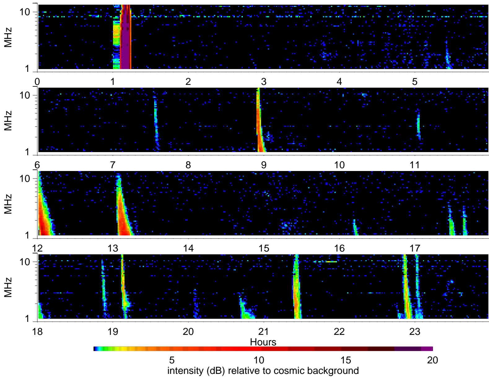
Wind Waves RAD2 receiver: 2000/2/7
