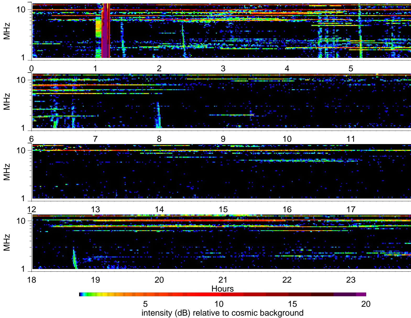
Wind Waves RAD2 receiver: 2000/2/1
