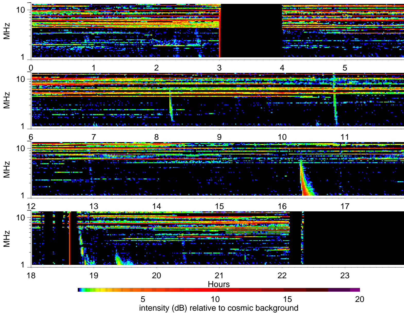
Wind Waves RAD2 receiver: 2000/1/27
