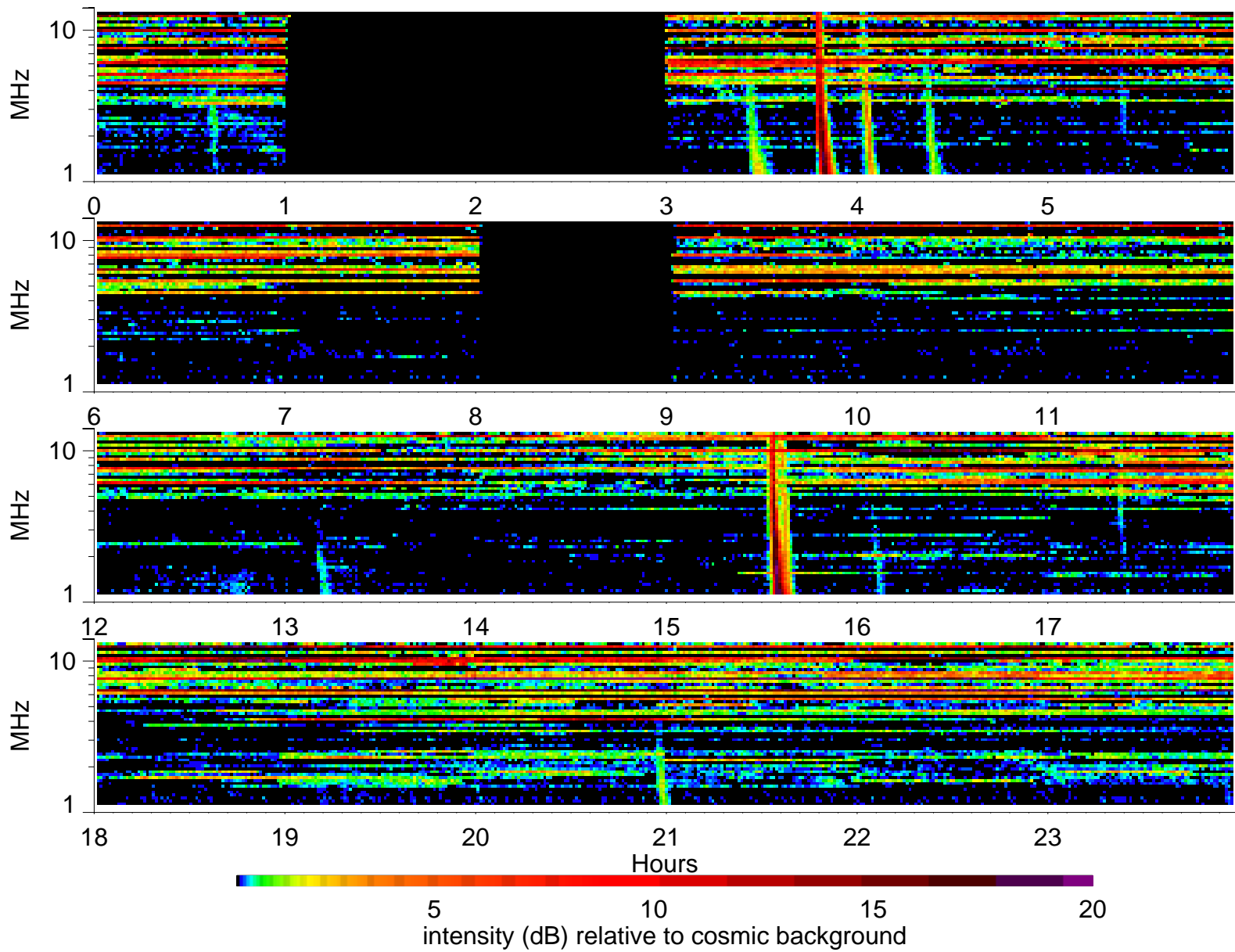
Wind Waves RAD2 receiver: 2000/1/25
